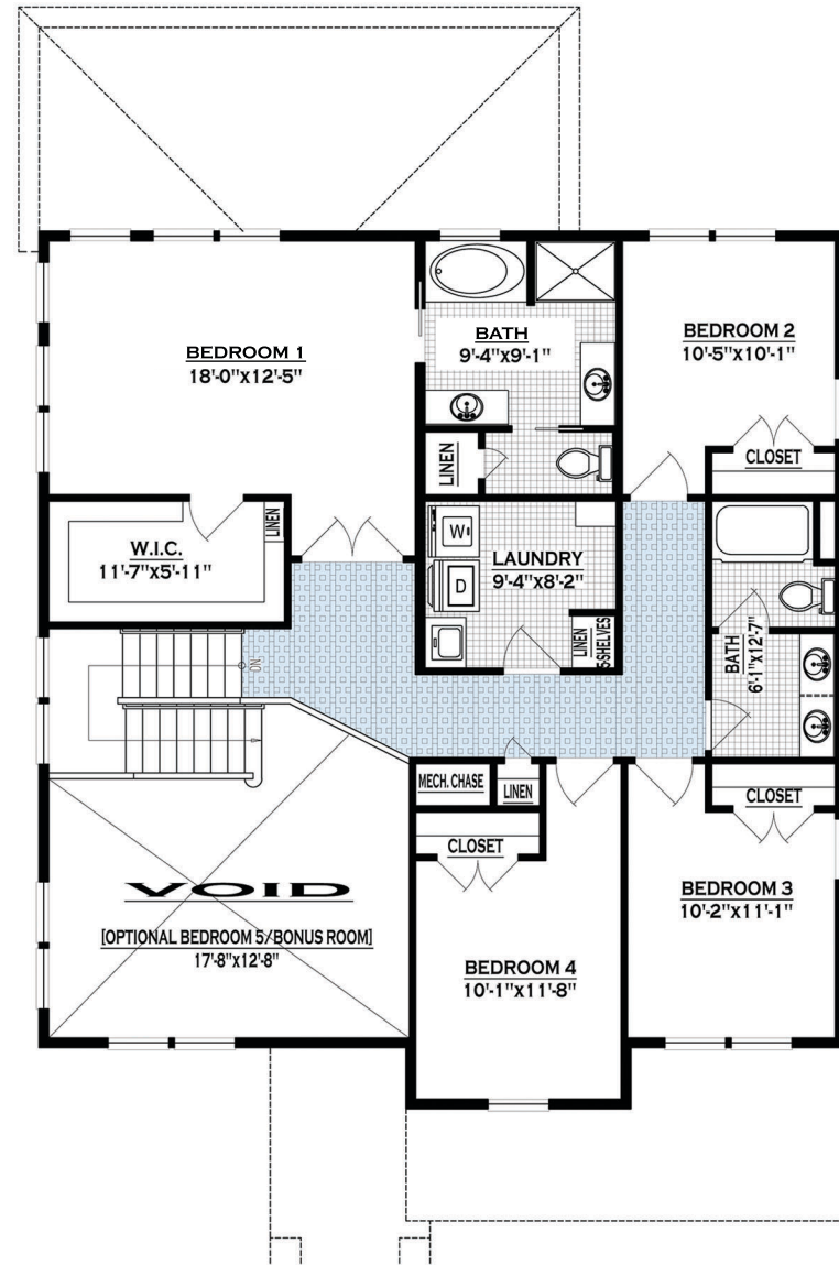
2ND. FLOOR PLAN
