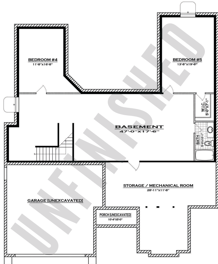
BASEMENT PLAN 2,159 SQ. FT.
