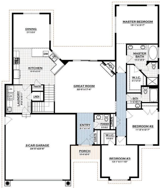
GROUND FLOOR PLAN 2,159 SQ. FT.
